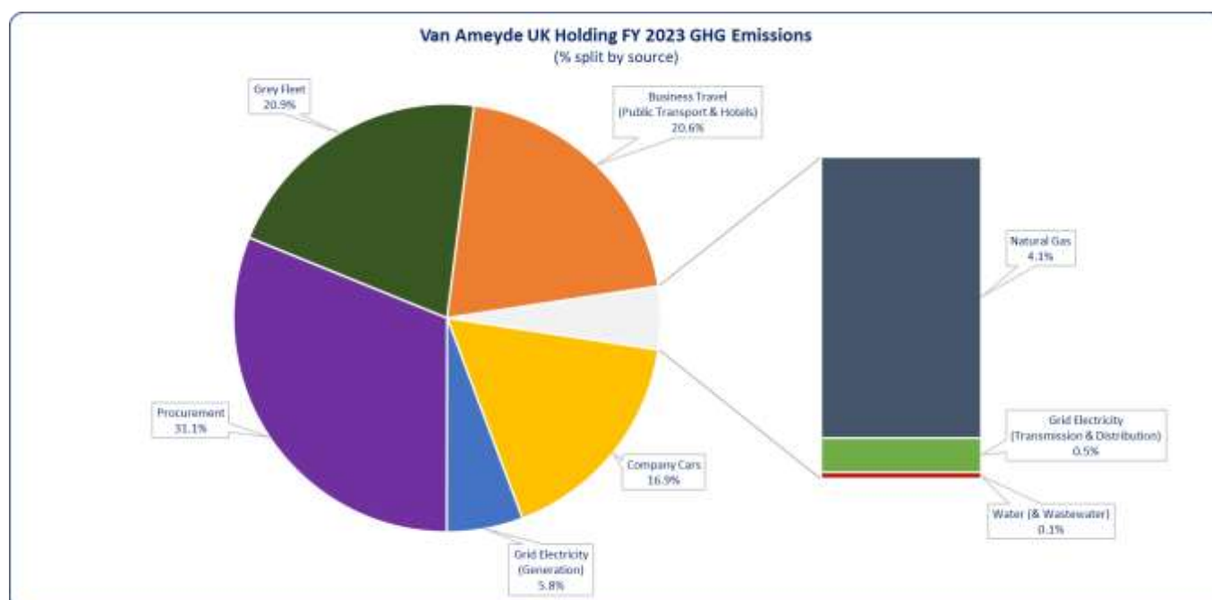
Figure 1 - Split of FY 2023 GHG emissions by source.
