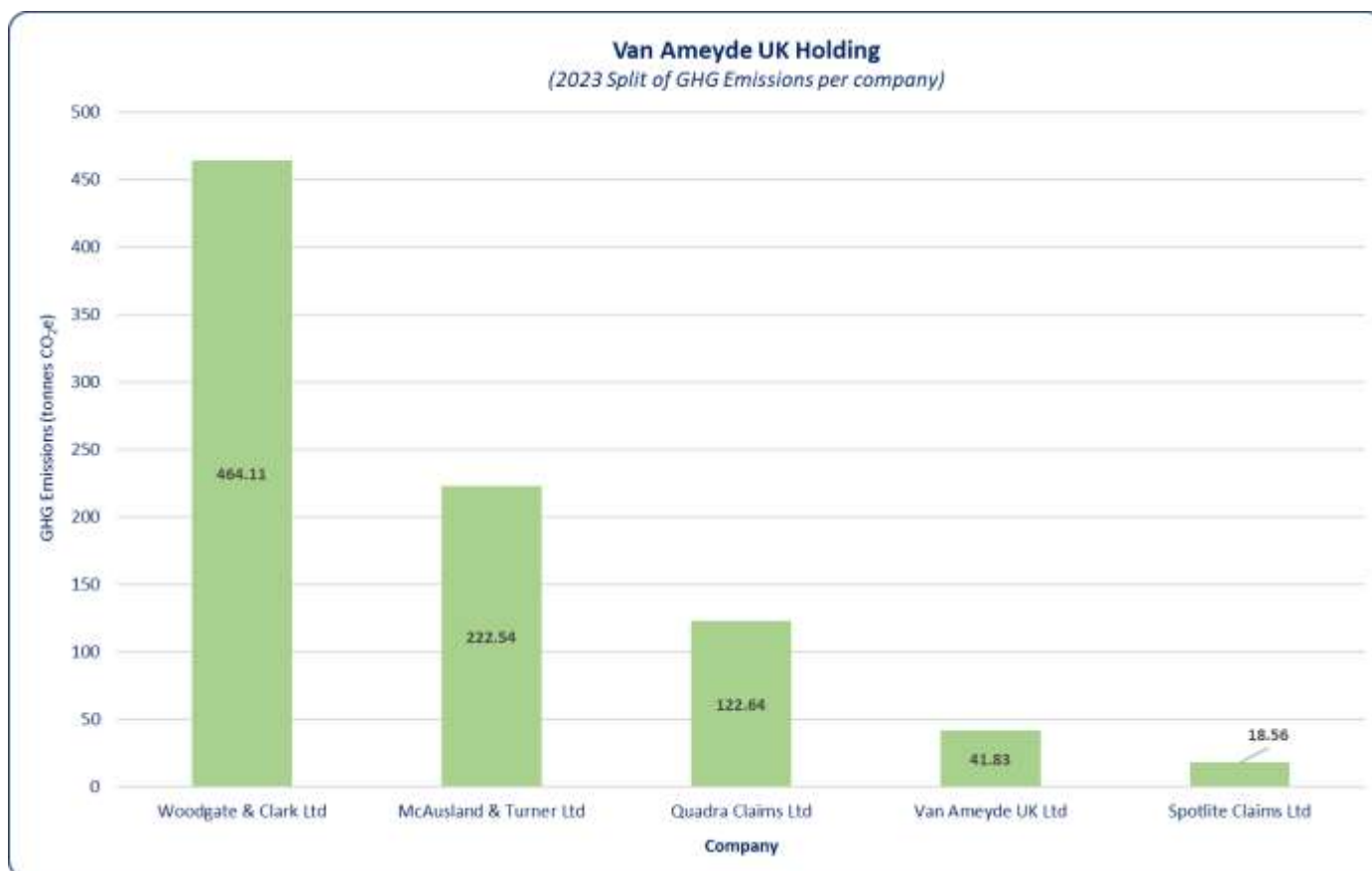
Figure 2 - Split of FY 2023 GHG emissions per company.
